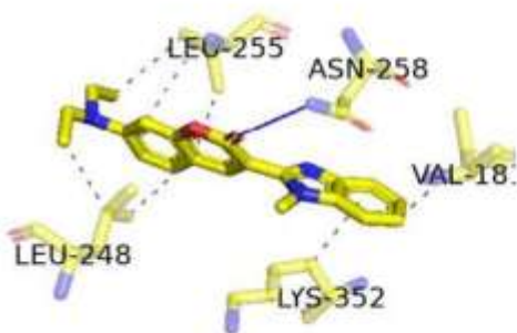
a) Coumarin-30
