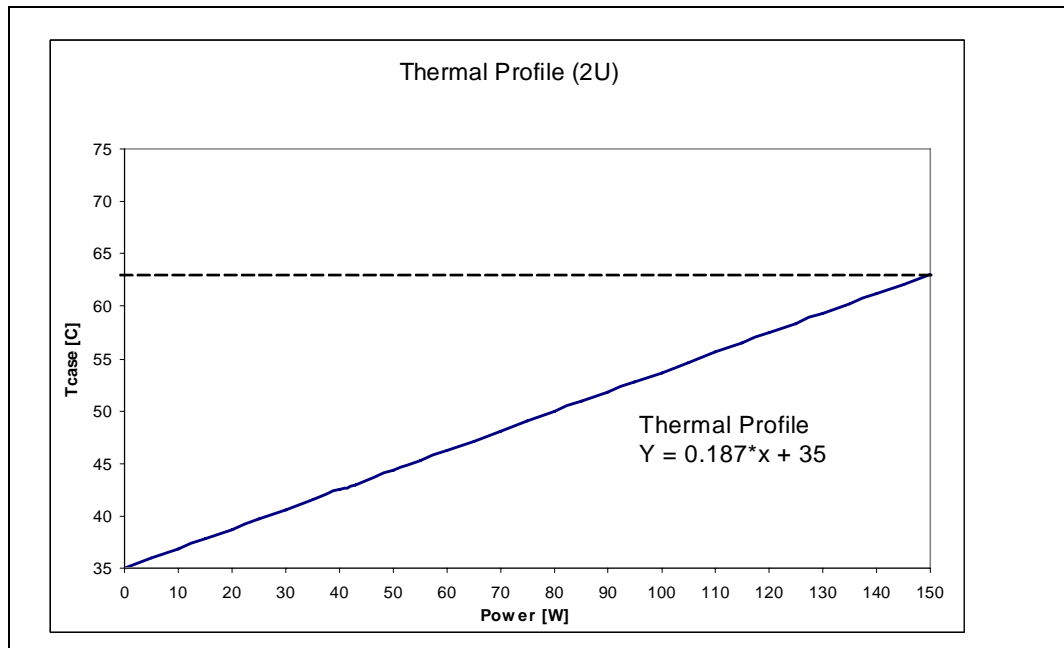
Figure 6-1. Quad-Core Intel® Xeon® Processor X5482 Thermal Profile
