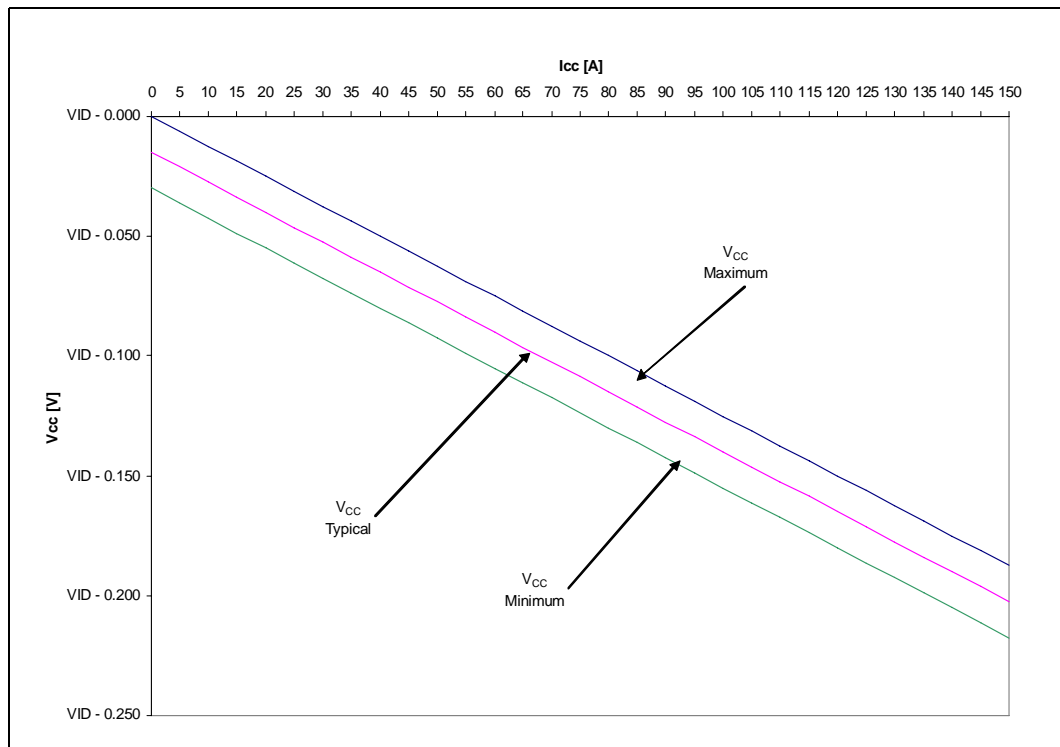
Figure 2-5. Quad-Core Intel® Xeon® Processor X5482 V CC Static and Transient Tolerance Load Lines
