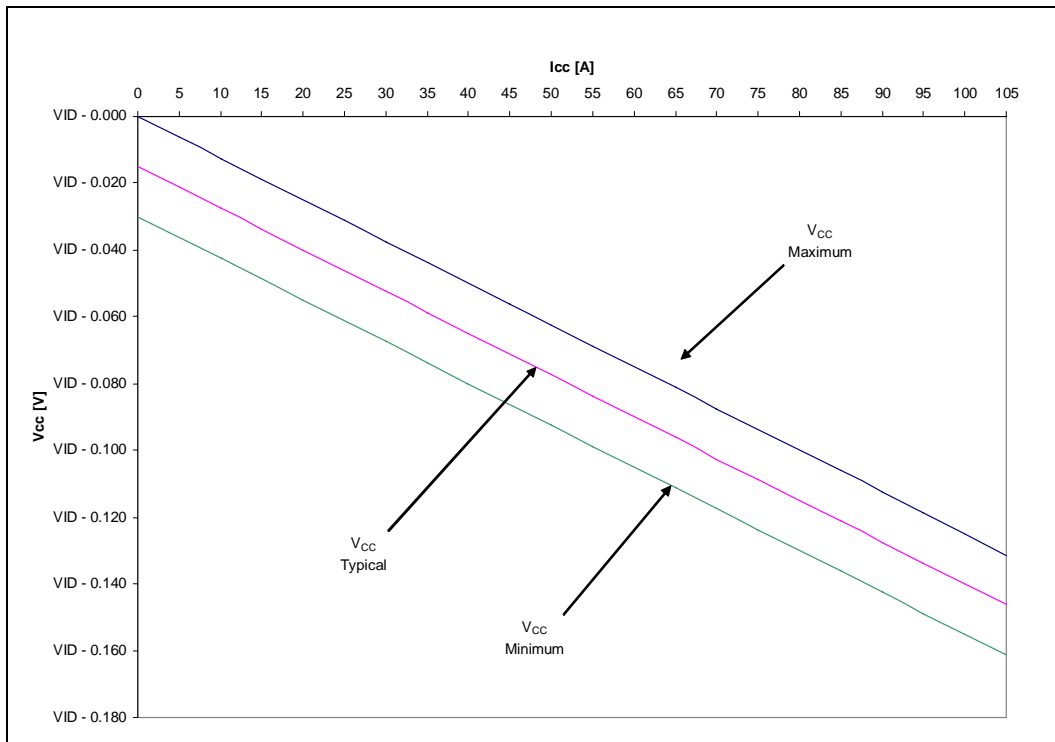
Figure 2-7. Quad-Core Intel® Xeon® Processor E5400 Series V_{CC} Static and Transient Tolerance Load Lines
