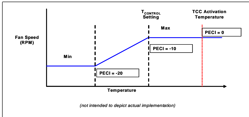
Figure 6-8. Conceptual Fan Control Diagram of PECI-based Platforms
