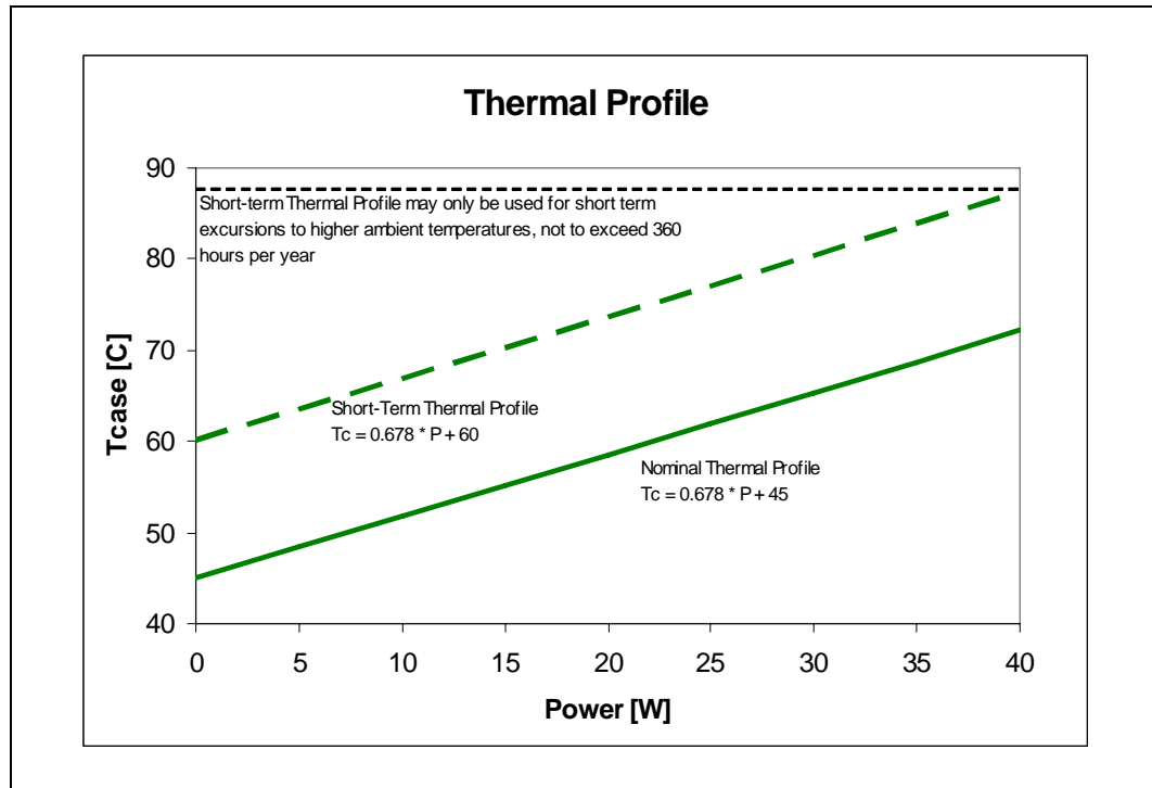
Figure 6-4. Quad-Core Intel® Xeon® Processor L5408 Thermal Profile
