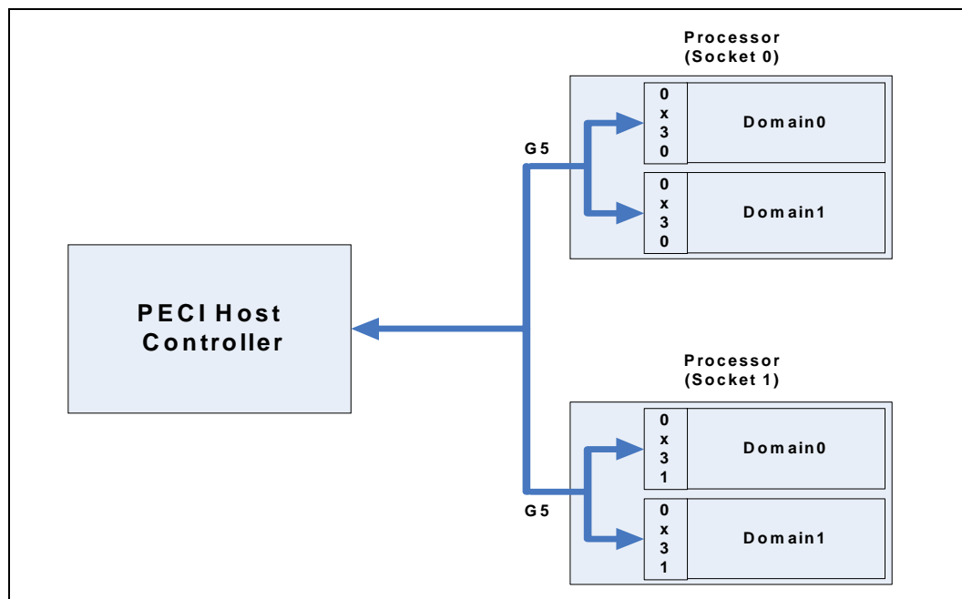
Figure 6-7. Quad-Core Intel® Xeon® Processor 5400 Series PECI Topology
