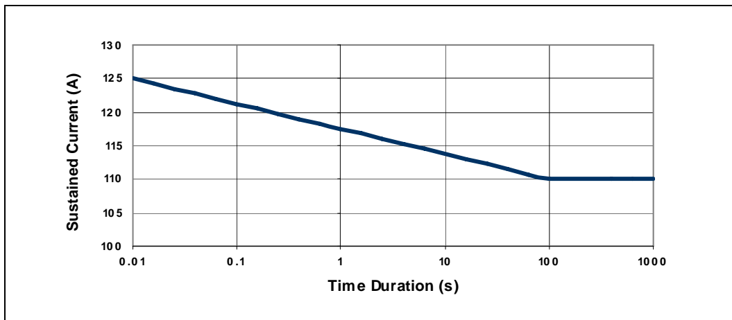
Figure 2-3. Quad-Core Intel® Xeon® Processor X5400 Series Load Current versus Time
